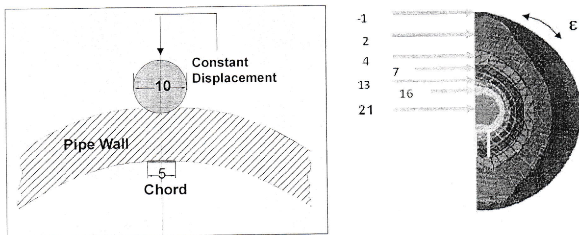
Figure 1: External point load at the pipe wall and finite element analysis of the elongation at the inside pipe wall
